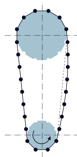
Vertical arrangement of the sprockets (unfavorable)
