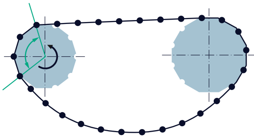
Enveloping angle
