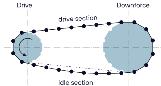
Horizontal configuration with the load located at the top (cost-effective)
